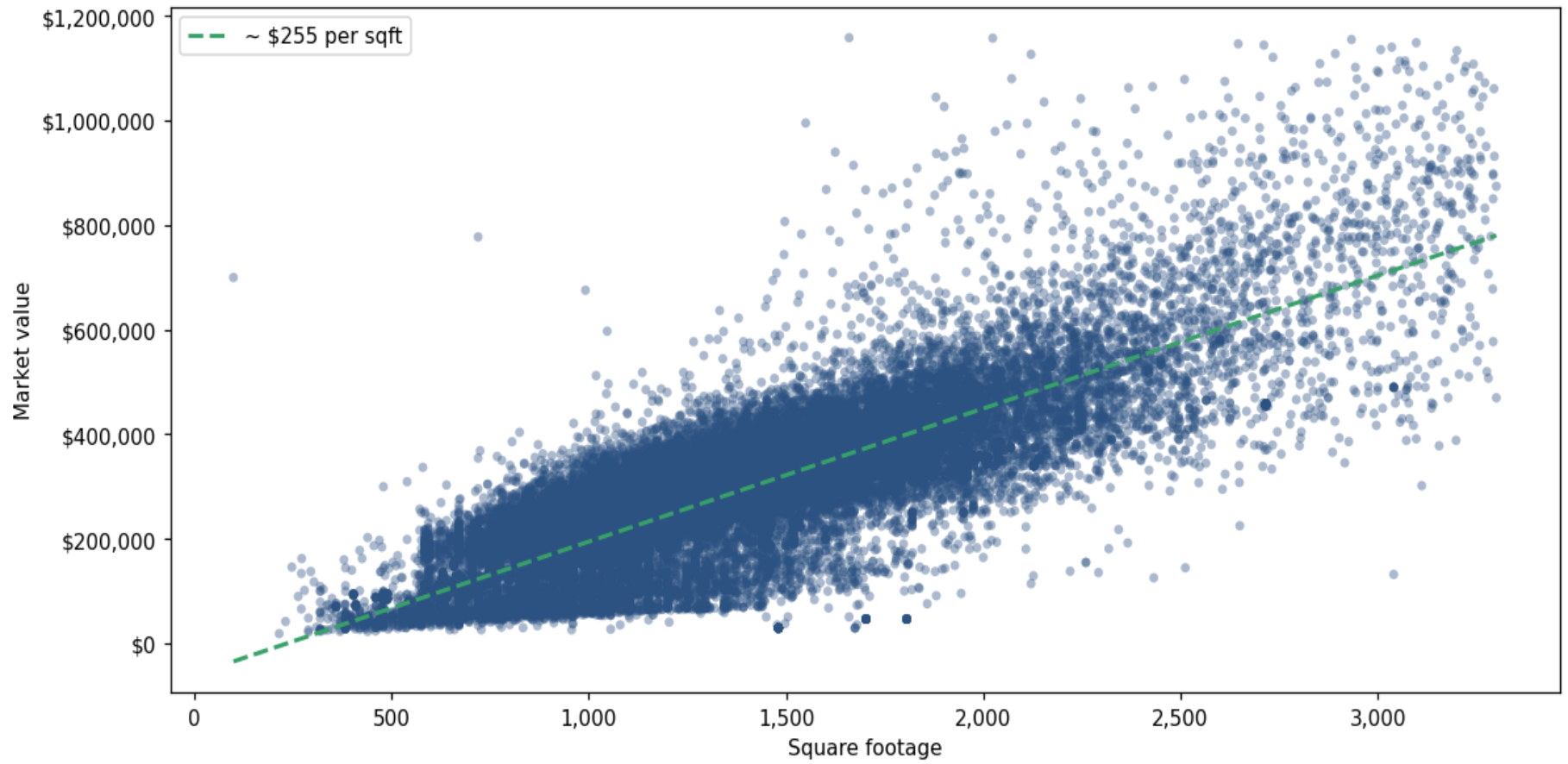
Building size vs. market value (n=35,765, outliers trimmed)
