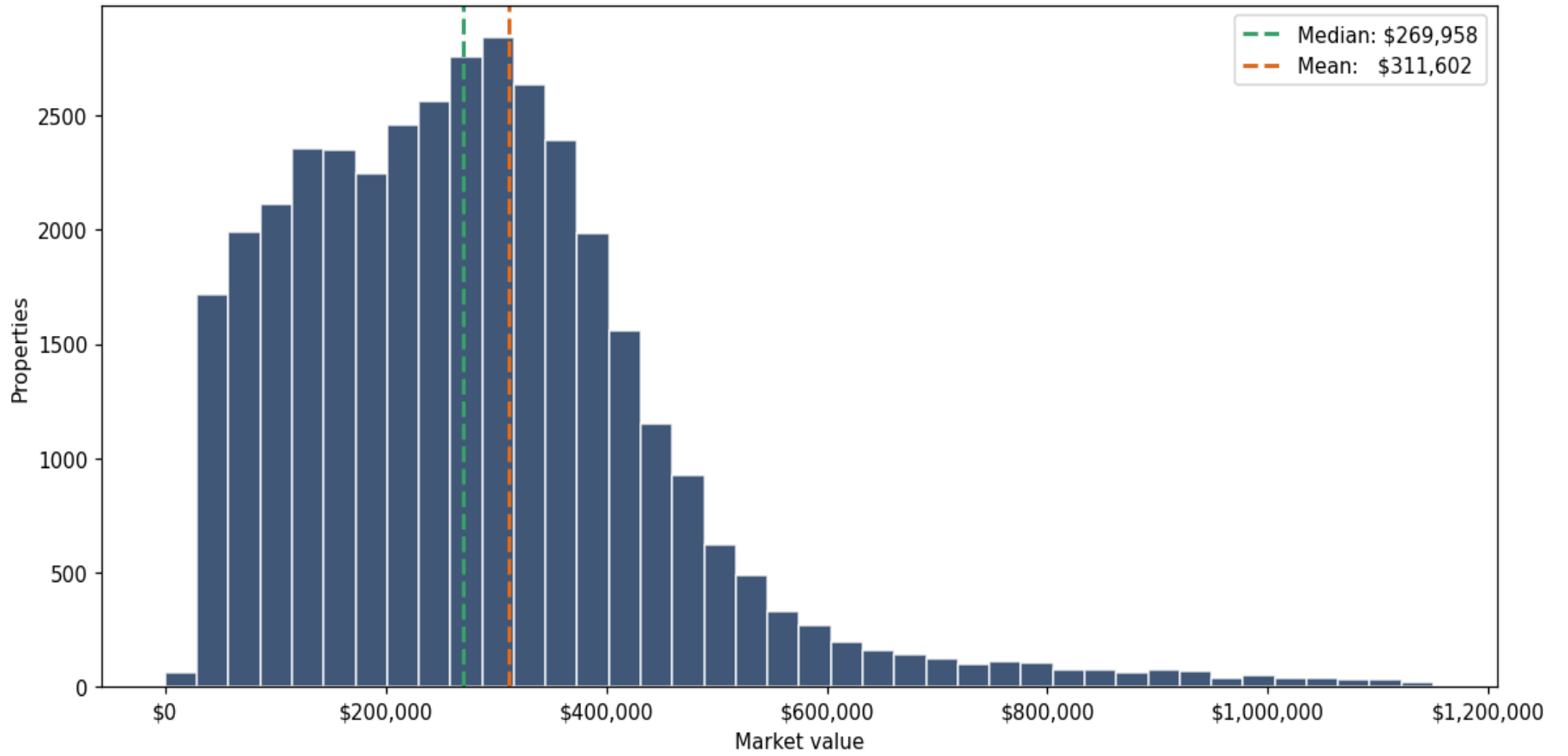
Market value distribution (n=37,721, top 1% trimmed for readability)
